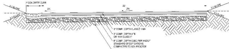
2 DRIVEWAY SECTION SCALE: NONE
