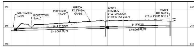
1 STORM PROFILE SCALE: H: 1"=20' V: 1"=5'
