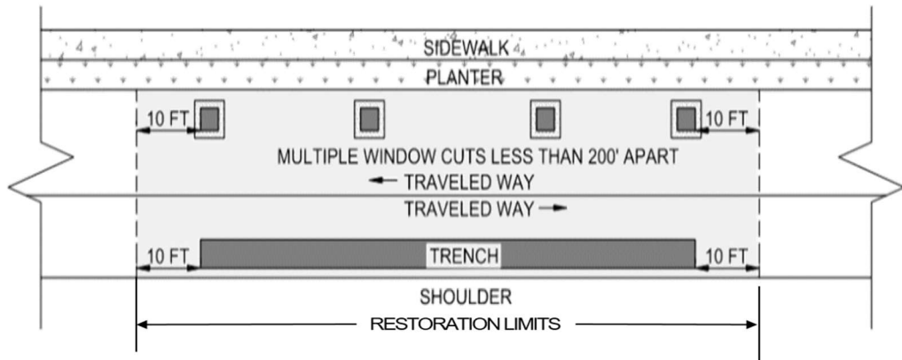
Figure 8 - 2 Full-Width Overlay Limits for Longitudinal Trenches and/or Multiple Window Cuts
