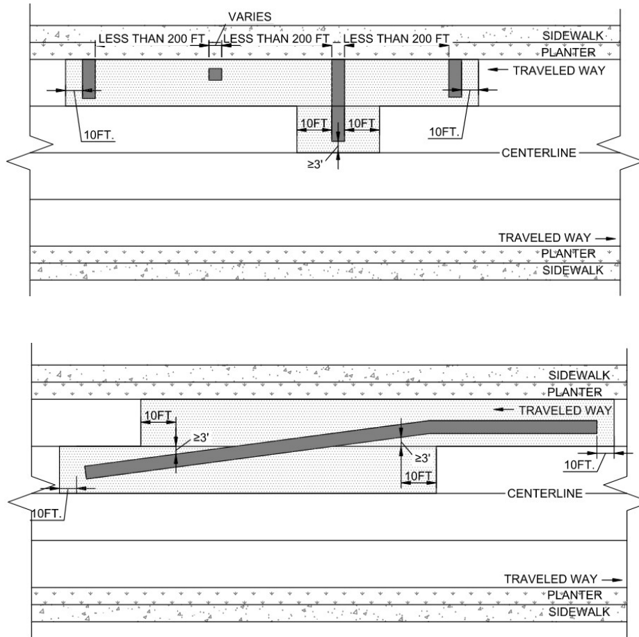
Figure 8 - 5 Overlay Limits for Pavement Cuts that Cross from One -Lane to Another
