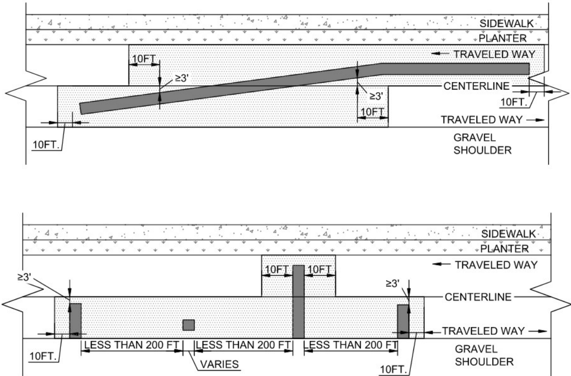
Figure 8 - 4 Overlay Limits for Trenches Within 3 Feet of the Crown of the Road
