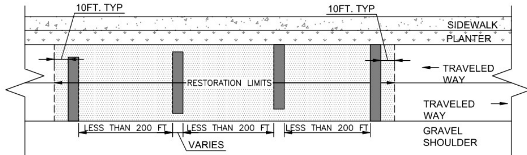
Figure 8 - 3 Full-Width Overlay Limits for Multiple Lateral Trenches
