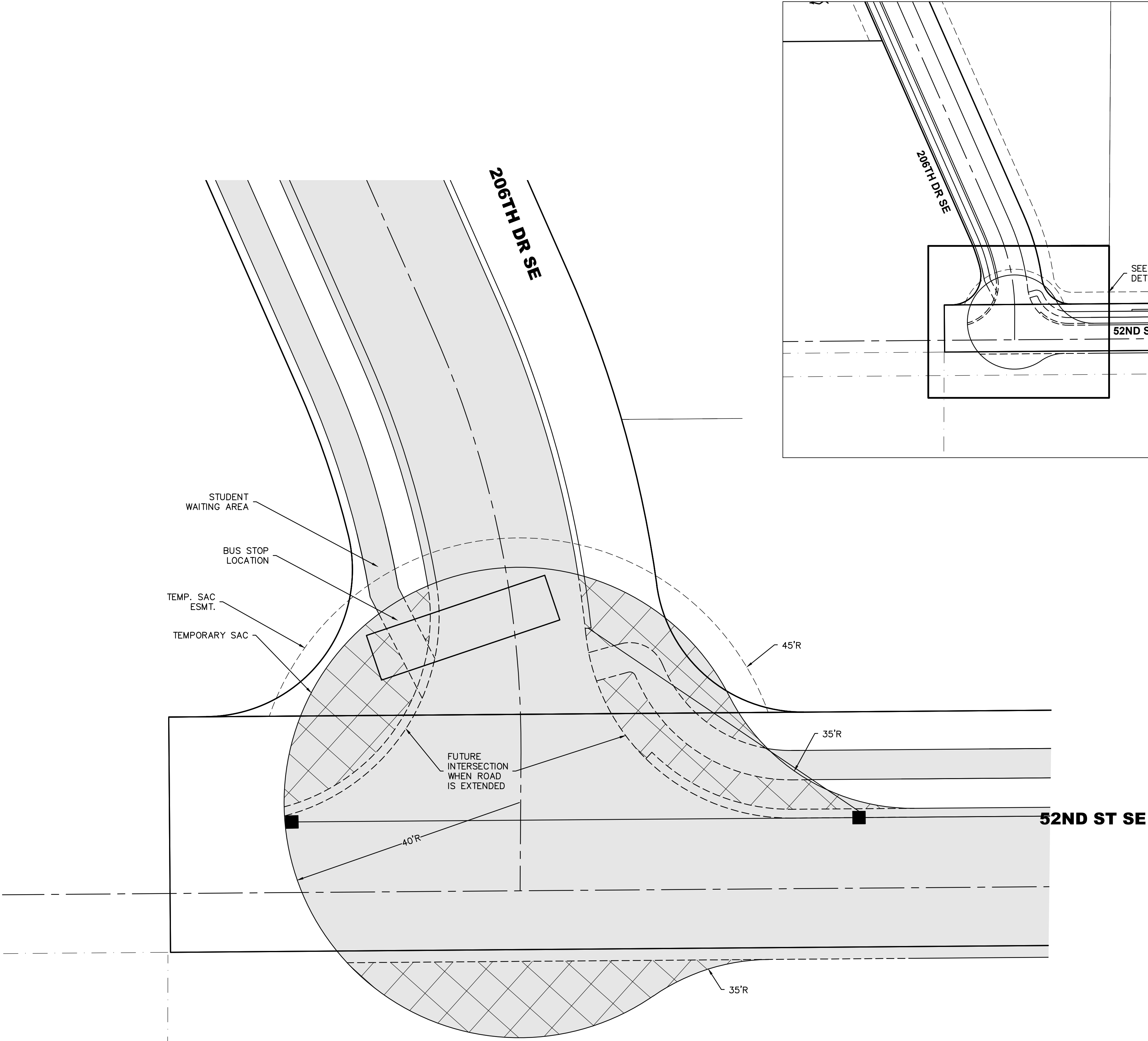
TEMPORARY CUL-DE-SAC
